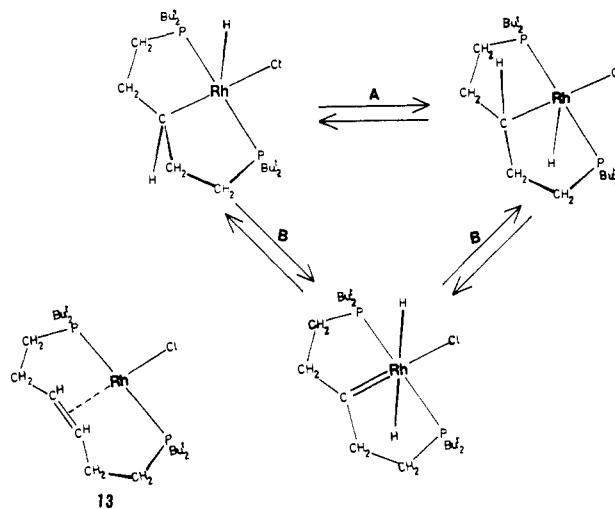
Scheme I. Possible Mechanisms to Explain the Fluxionality of 6: (A) A Concerted Process Requiring a Transoid Arrangement of H-C-Rh-H and a Vacant Orbital on the Rhodium; (B) Stepwise, or Carbenoid (Ylide) Mechanism
