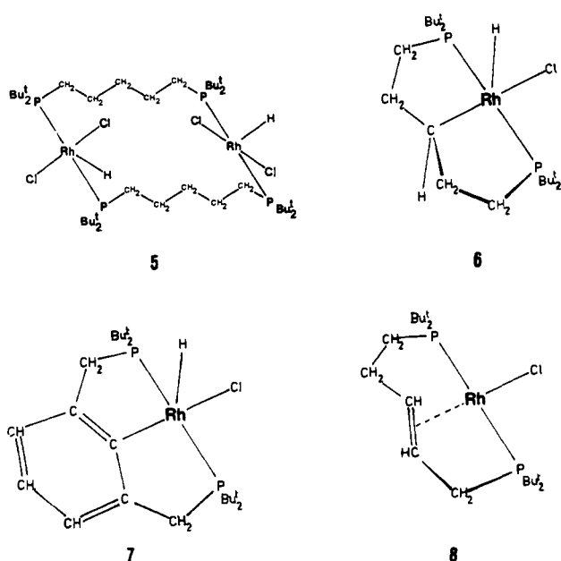
Scheme I. Possible Mechanisms to Explain the Fluxionality of 6: (A) A Concerted Process Requiring a Transoid Arrangement of H-C-Rh-H and a Vacant Orbital on the Rhodium; (B) Stepwise, or Carbenoid (Ylide) Mechanism
